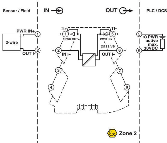
Figure 3 Block diagram
