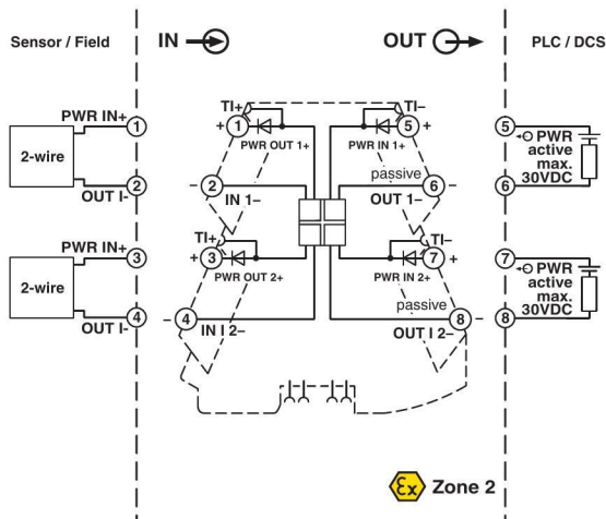
Figure 4 Block diagram
